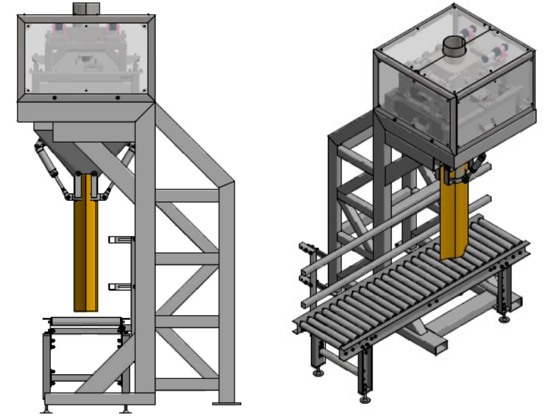
25 kg Bag Filling Machine
