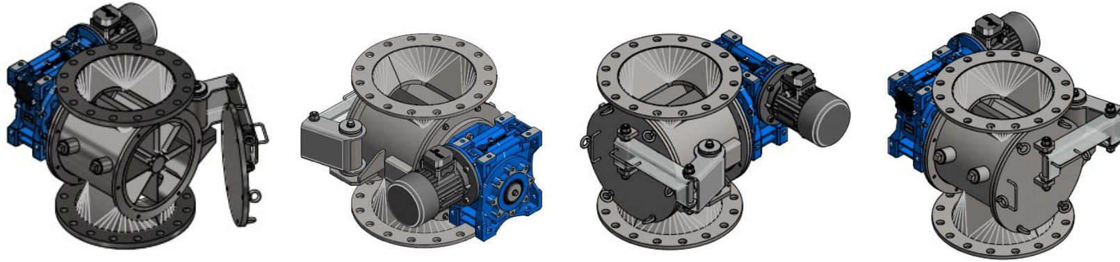
Air Lock Rotary Valve, Compact Type, Easy Clean Series
