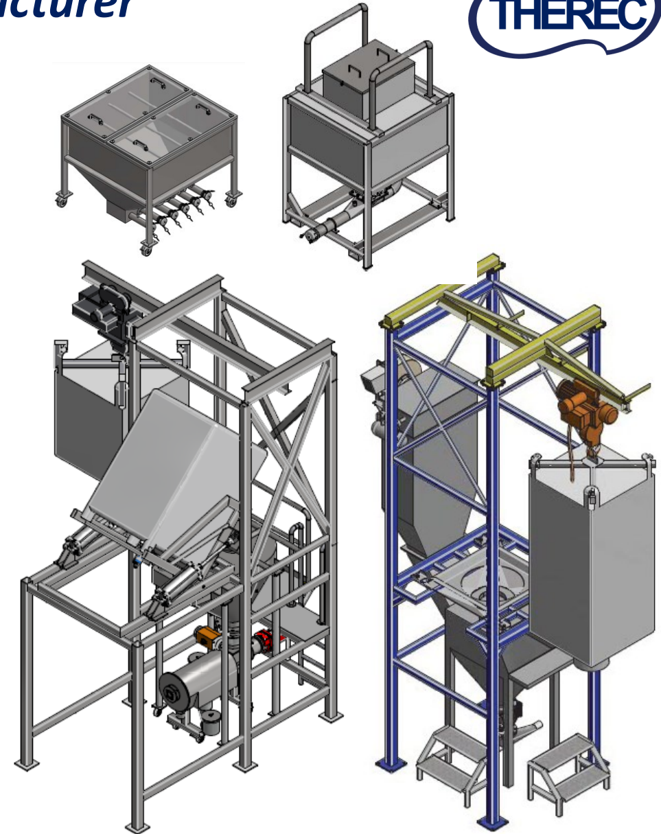
Bag & Bin Unloading Station
